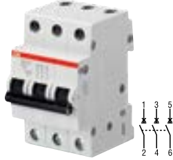
SH203T-B
