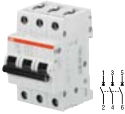
S203M-B16
