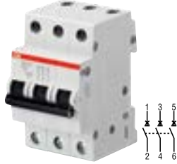
SH203 T-C 6
